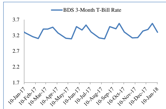
Figure 2 - BDS 3-Month T-Bill Rate
